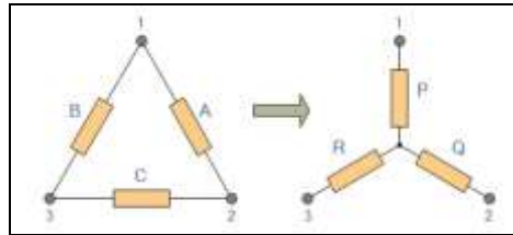
Fig. 1. Delta to Star conversion.
